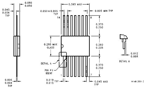
14-Lead Ceramic Flat Package (W) Order Number 54LS20FMQB or DM54LS20W NS Package Number W14B
